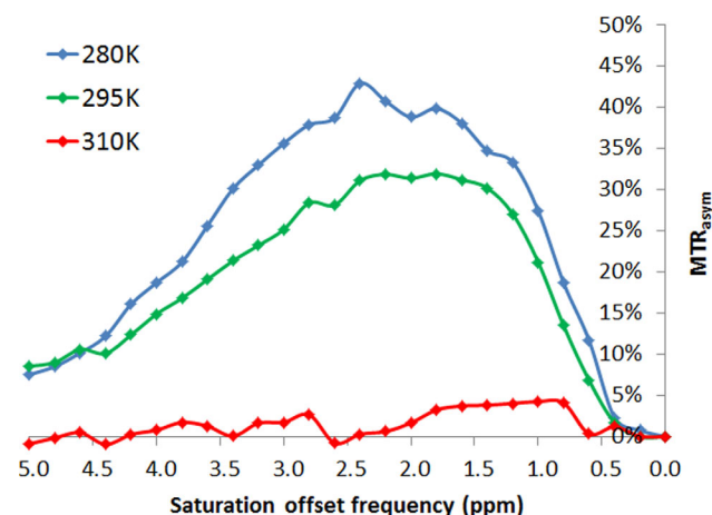
FIG. 2. \text{MTR}_{\text{asym}} plots from z-spectra acquired from 20 mM solutions of spermine at pH 6.5. The increasing CEST effect at lower temperature (reducing k_{sw} ) indicates chemical exchange in the intermediate-to-fast regime at T = 310 K
