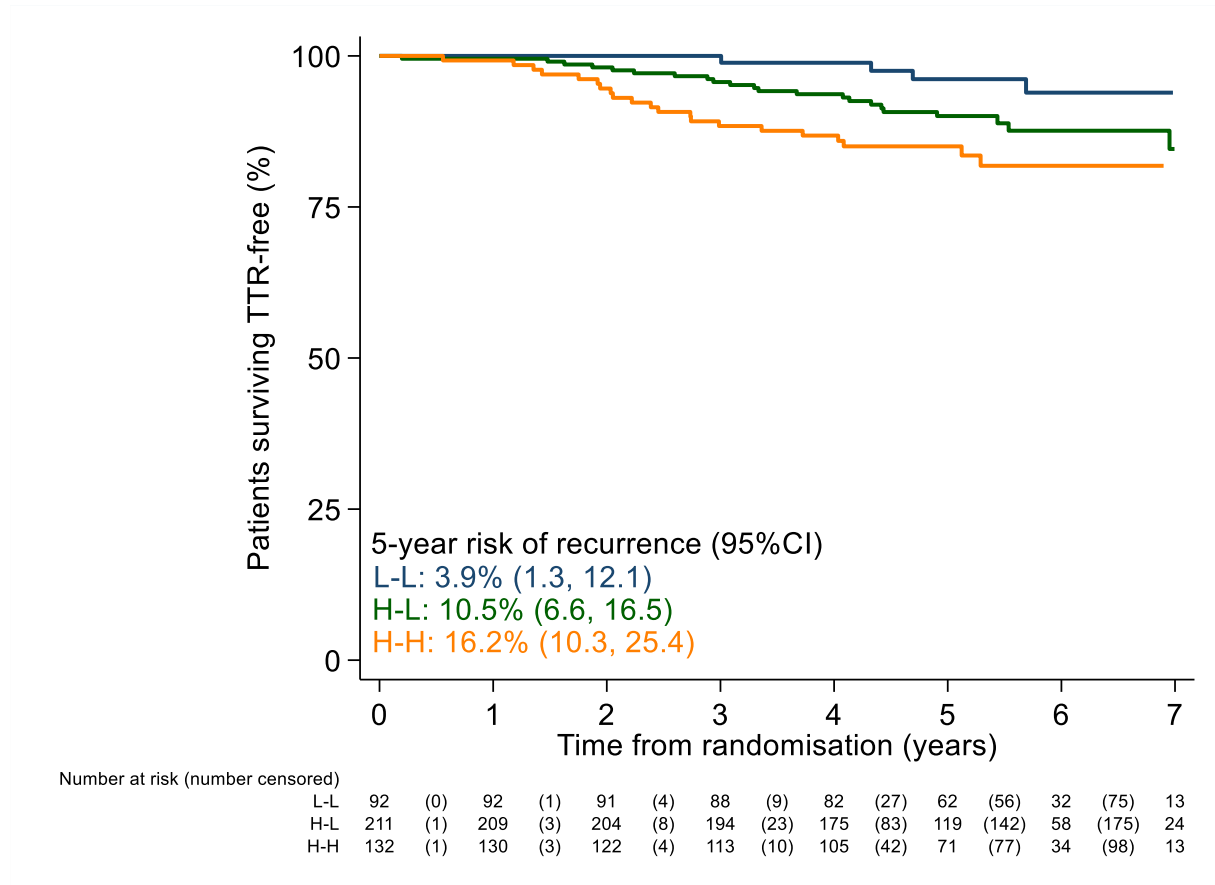
Figure A3a: Kaplan Meier survival curve for time to recurrence by Ki67_B and Ki67_{2W} for patients with HR+ and HER2-negative breast cancer allocated perioperative AI who are <70 years old and received chemotherapy (N=442)
