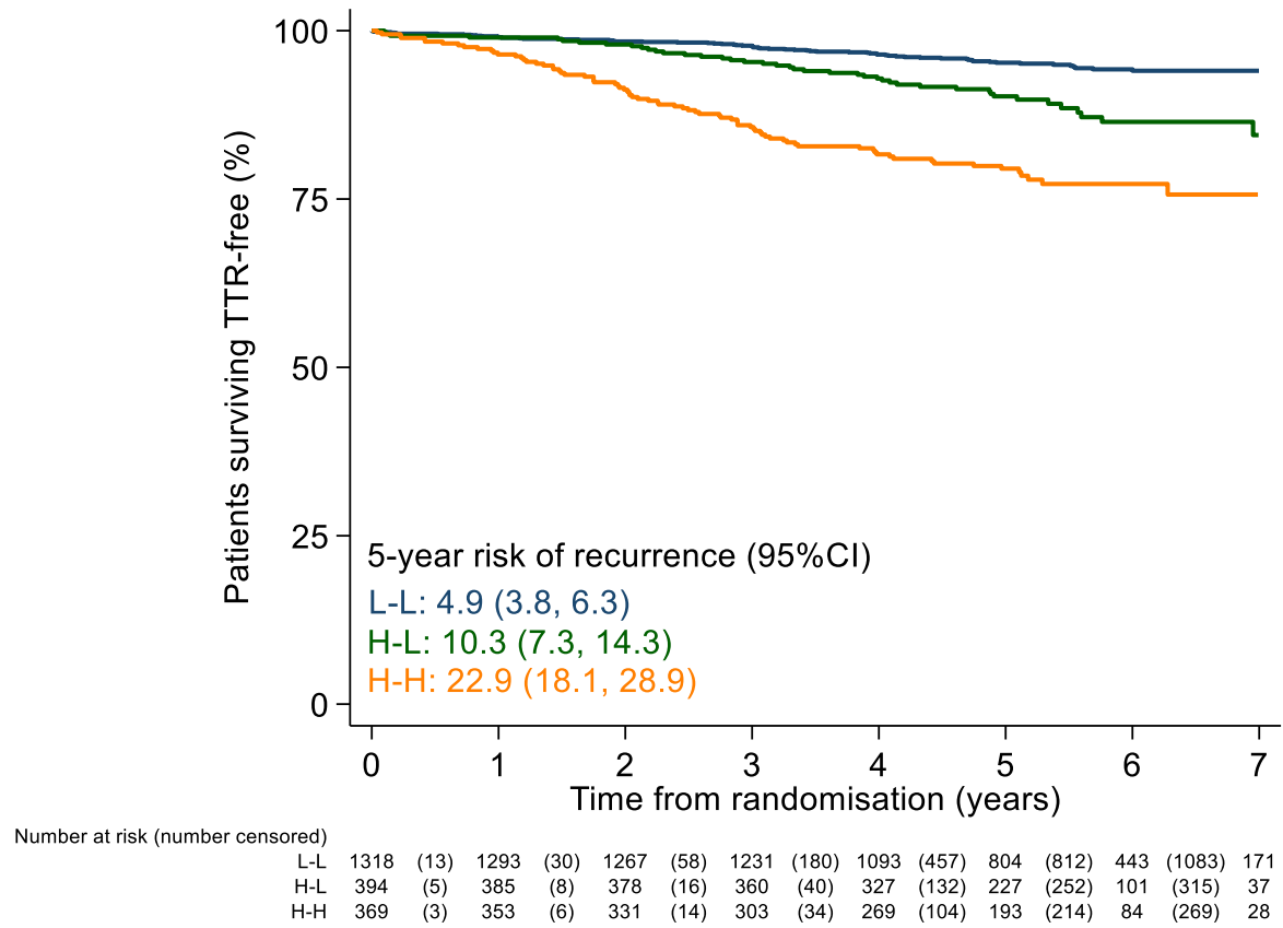
Figure A6b: Exploratory analysis using Ki67 B (20% cut-point) and Ki67 2W (8% cut-point) for patients with HR+ and HER2-negative breast cancer allocated perioperative AI - Kaplan Meier survival curve for time to recurrence by Ki67 B and Ki67 2W
