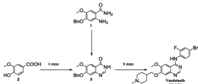
Scheme 1. Current synthetic procedure to Vandetanib via the key quinazolinone intermediate 3.
