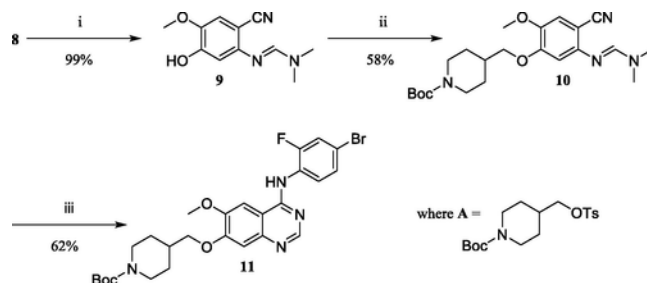
Scheme 3. Reagents and conditions: i) TFA, microwave (max. power 400 W), 70 °C, 45 min; ii) A, Cs 2 CO 3 , MeCN, reflux, 3 hr; iii) 4-bromo-2-fluoroaniline, 130 °C, 1 h.
