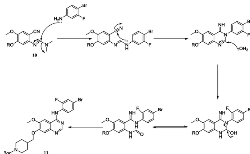
Scheme 4. Proposed mechanism for the Dimroth rearrangement; derived from Chandregowda and co-workers in their synthesis of Erlotinib and Gefitinib. 16
