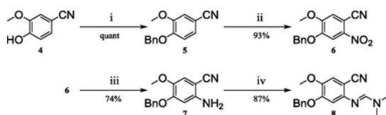
Scheme 2. Reagents and conditions: i) Benzyl bromide, K 2 CO 3 , DMF, rt, 18 h; ii) Nitric acid, Ac 2 O, 0 °C to rt, 18 h; iii) NaHCO 3 , tetra-butyl ammonium chloride, Sodium dithionite, DCM, water, rt, 2 h; iv) DMF-DMA, microwave, 90 °C, 15 min.
