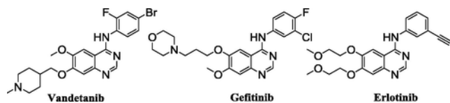
Fig. 1. Structures of Vandetanib (Caprelsa™), Gefitinib (Iressa™) and Erlotinib (Tarceva™).
