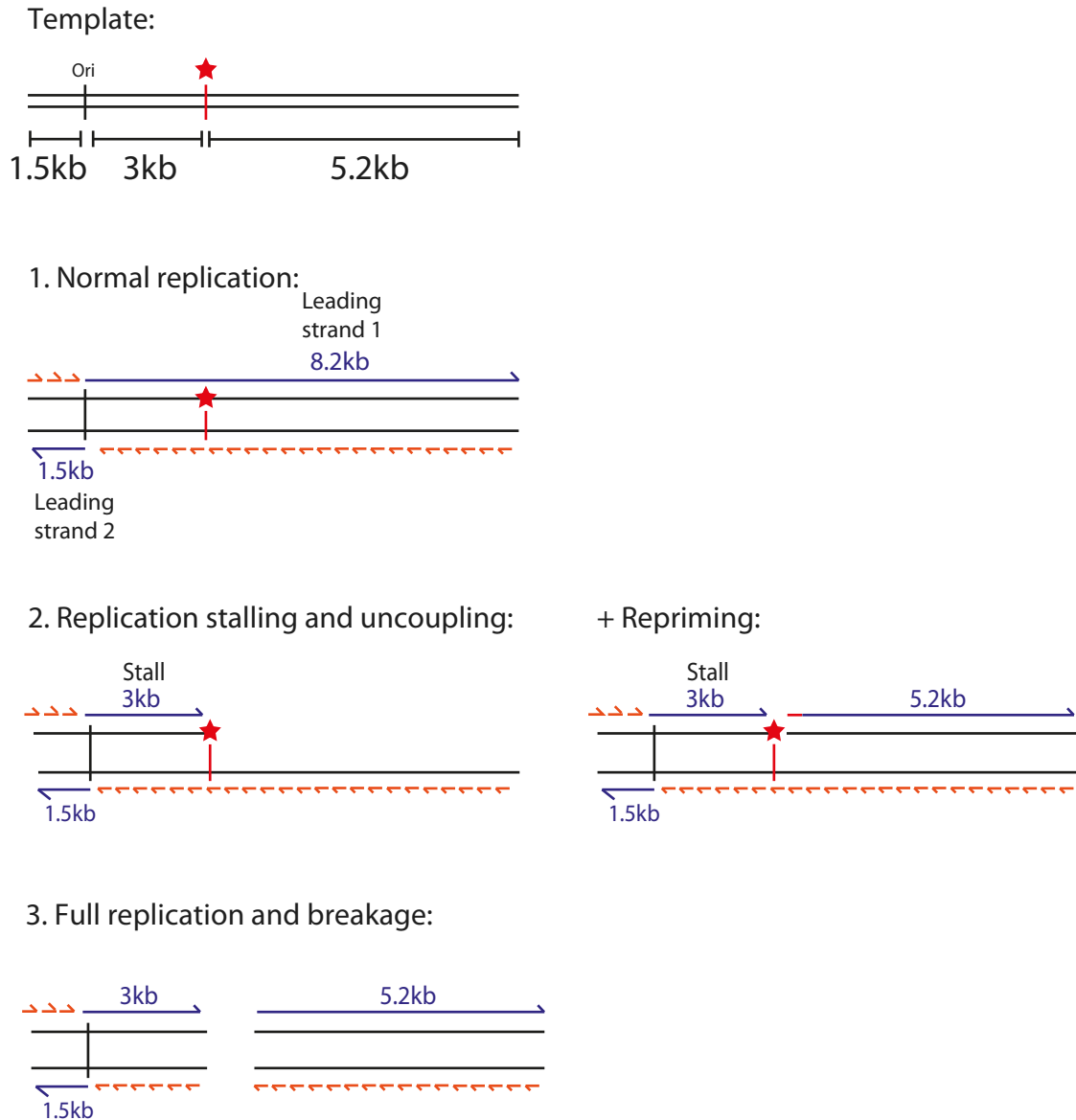
Figure EV1. Schematic of potential replication products from G4 and iM-containing templates.
