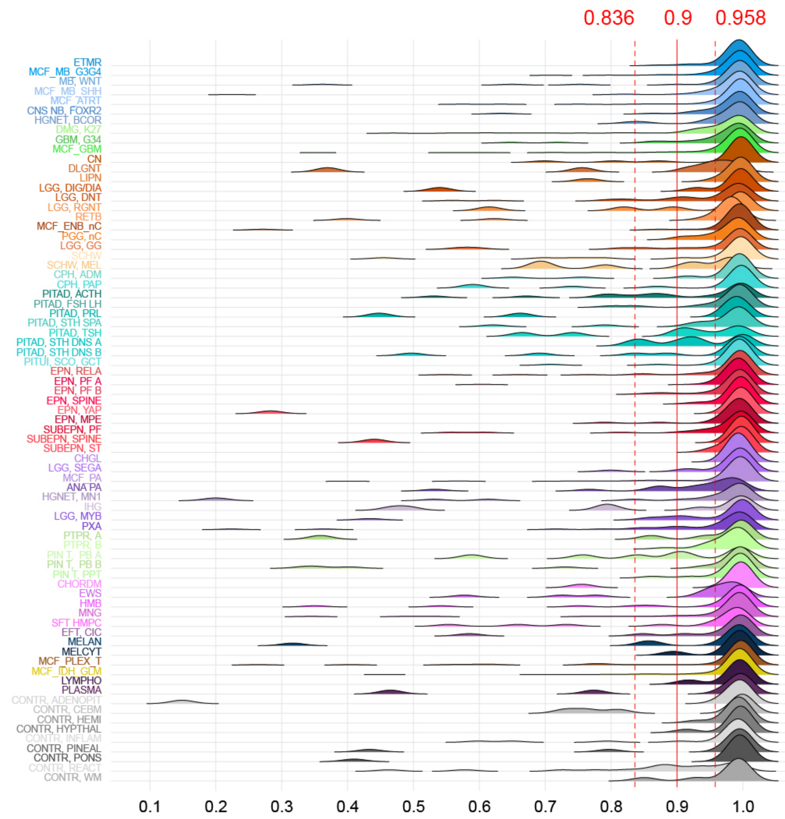
Calibrated scores for correctly classified cases
