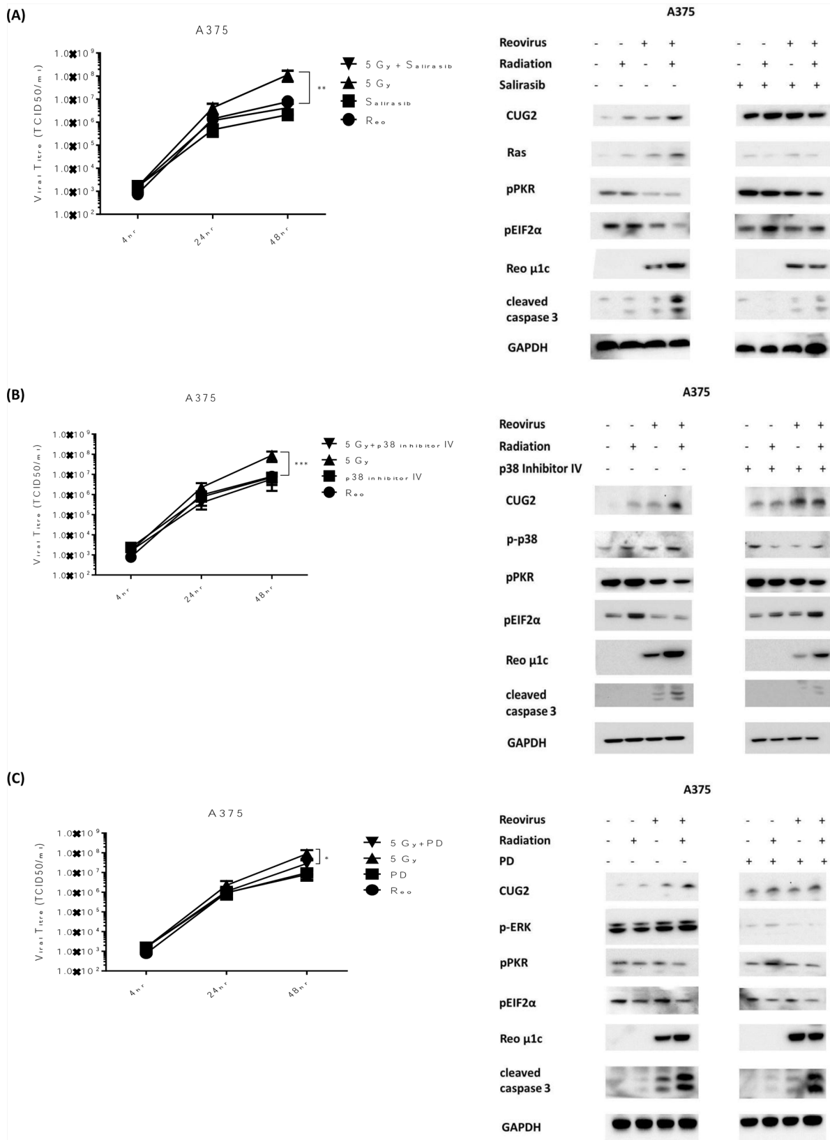
Figure 4: RT-induced viral replication is reversed by inhibition of either Ras or p38. A375 cells were treated with salirasib (10 \mu M) A , p38 inhibitor IV (10 \mu M) B , or PD184352 (1 \mu M) C , 1hr before irradiation at 5 Gy and 5 hrs before infection with RT3D (MOI 5). Viral titres were assessed by one - step growth curve assays (A-C). Protein was isolated at 48hrs and expression of CUG2, pPKR, p-eIF2 \alpha , cleaved caspase 3 and viral protein \mu 1c were detected by western blotting (A-C). Expression of Ras (A), p-p38 (B) and pERK (C) were also assessed.
