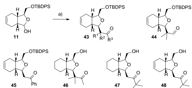
Scheme 6. Reagents and Conditions: a) Silyl enol ether, BF 3 ·OEt 2 (TMSOTf for 46 ), CH 2 Cl 2 , -78 °C 36–97%.
