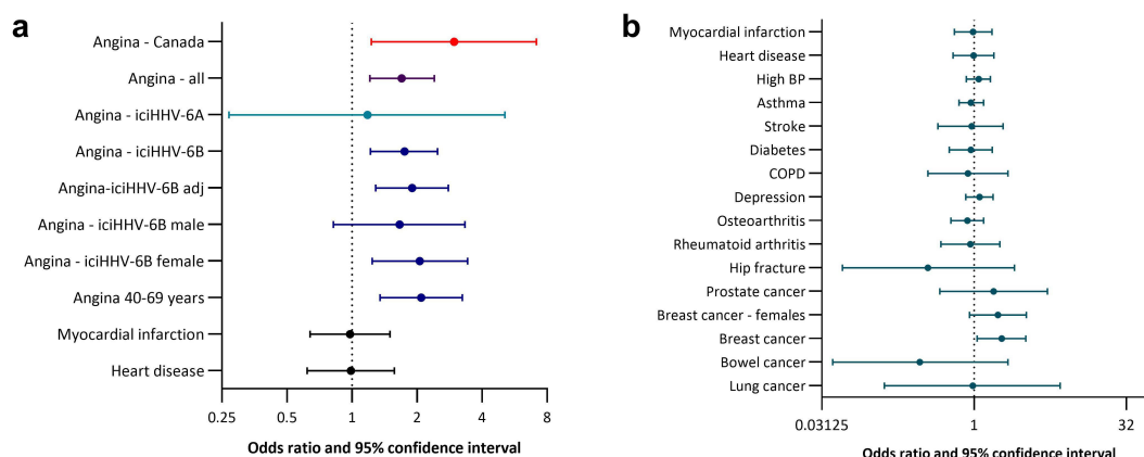
FIG 2 Association between icHHV-6 and diseases forest plots showing OR and 95% CIs for risk of angina and other conditions with data available at baseline (date of recruitment). (a) Association between icHHV-6B and angina. Angina - Canada: the adjusted OR and 95% CIs from the CARTaGENE study (30) are shown for comparison. Angina - all: icHHV-6A and icHHV-6B combined, adjusted for age and sex. Angina - icHHV-6A and Angina - icHHV-6B: data by viral species, adjusted for age and sex. Angina - icHHV-6B adj: analysis adjusted for age, sex, body mass index, average systolic blood pressure, body fat, nationality, Scottish Index of Multiple Deprivation (quintiles), and smoking status. Angina - icHHV-6B male, Angina - icHHV-6B female, and Angina 40–69 years (the age range in the CARTaGENE study) are adjusted for the variables included in icHHV-6B adj. Adjustments for age include age as a continuous variable. (b) Association between icHHV-6 and 15 conditions with baseline data. COPD, chronic obstructive pulmonary disease. Data for Parkinson's disease are not shown as there were no icHHV-6-positive individuals with Parkinson's disease.
