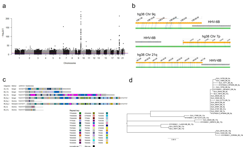
FIG 3 HHV-6 integrations and ancestral viral lineages. (a) Manhattan plot showing an association between icHHV-6B and imputed genetic variants close to the telomeres of chromosome 7p, 9q, 11p, 17p, and 19q. (b) Analysis of samples with clade B6 icHHV-6B genomes by optical genome mapping. Consensus maps (cmaps, green bars) from optical genome mapping were assembled using the human genome (hg38 build, yellow bar) as a reference on the basis of fluorescent labeling of CTTAAG recognition sites that aligned to the human reference (blue vertical lines) or did not align to the human reference (red vertical lines). The pattern of fluorescent labels unique to the HHV-6B genome (gray bar) could be identified in unaligned fluorescent labels at the ends of cmaps that aligned to chromosome 7 p, 9q, and 21q for GLA_21713, GLA_32597, and GLA_13910, respectively. (c) Patterns of telomere and telomere-like repeats in the junction fragment between icHHV-6 and low copy-number sequence in the subtelomere. Each small rectangle represents a telomere or telomere-like sequence as indicated in the Repeat key. * Denotes an omitted telomere-repeat array of 290 hexamers, 65% TTAGGG interspersed with telomere-like repeat, almost entirely TTAGAC-CTAGGG dimers. B6_9q_1 refers to B6_9q_hap1 (B6_9q_T2), B6_9q_2 refers to B6_9q_hap2 (B6_9q_T1). (d) Evolutionary analysis by Maximum Likelihood method of 20 icHHV-6B genome sequences from GS:SFHS and seven publicly available icHHV-6B genome sequences. Branch tips are labeled with sample name and lineage, where known. The evolutionary history was inferred using the Maximum Likelihood method and Tamura-Nei model (51). Branch lengths are measured in the number of substitutions per site. There were a total of 140,246 positions in the final data set.
